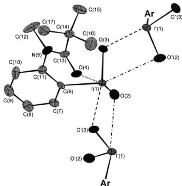
Figure 1. CAMERON drawing of a polymeric chain in the solid-state structure of 15e at the 30% probability level (hydrogen atoms are omitted for clarity, Ar = 2-C 6 H 4 NMeCO 2 tBu). Selected distances [Å] and angles [°]: I(1)–O(2) 1.791, I(1)–O(3) 1.832, I(1)⋯O''(2) 3.226, I(1)⋯O'(3) 2.627, I(1)–C(6) 2.115, I(1)⋯O(4) 2.647, N(5)–C(13) 1.349, O(4)–C(13) 1.225, O(2)–I(1)–O(3) 103.88, O(2)–I(1)–C(6) 99.01, O(3)–I(1)–C(6) 94.38, O(2)–I(1)⋯O(4) 166.31, C(6)–C(11)–N(5)–C(13) 41.33.
