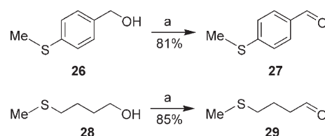
Scheme 4. Site-selective oxidation of thioalcohols 26 and 28 . a) 15d (1.0 equiv), MeSEt (1.0 equiv), DCE, reflux, 2.5 h.
