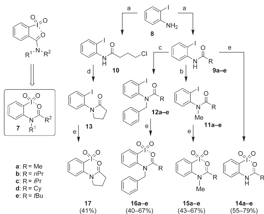
Scheme 2. Preparation of target aryl iodyl derivatives 14a–e , 15a–e , 16a–e , and 17 . a) RCOCl (1.0 equiv), Et 3 N (1.1 equiv), THF, 0°C→RT, 30 min; b) 1. NaH (1.1 equiv), THF, 0°C, 30 min; 2. MeI (1.3 equiv), THF, 0°C→RT, 3 h; c) 1. NaH (1.1 equiv), THF, 0°C, 30 min; 2. BnBr (1.3 equiv), THF, 0°C→RT, 3 h; d) NaH (1.1 equiv), THF, 0°C→RT, 3 h; e) 3,3-dimethyldioxirane (3.0 equiv, 0.1 M in acetone), CH 2 Cl 2 , 0°C→RT, 3 h. Cy=cyclohexyl.
