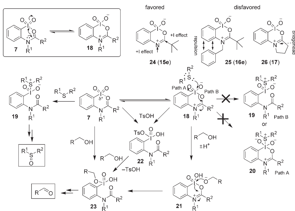
Scheme 3. Proposed mechanistic rationale for the reactivity of pseudo-benziodoxazines 14–17 towards alcohols and sulfides. I effect = inductive effect.
