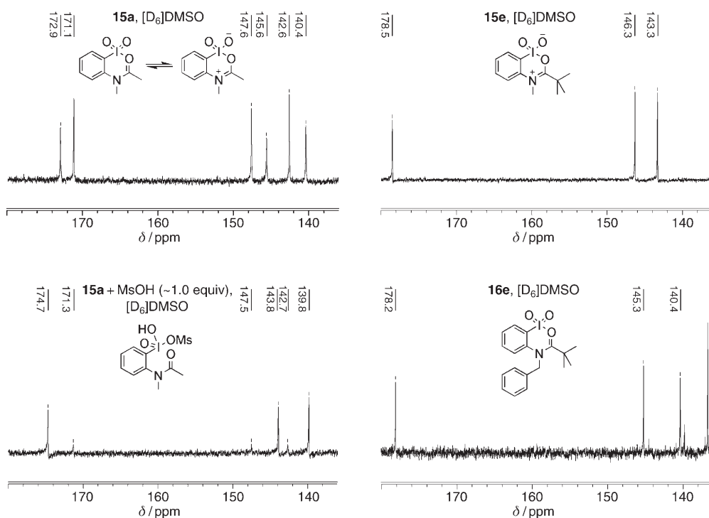
Figure 2. 13 C NMR spectra ( \delta = 136–180 ppm) of iodylarenes 15a , 15a + MsOH (1.0 equiv), 15e , and 16e in [D 6 ]DMSO.
