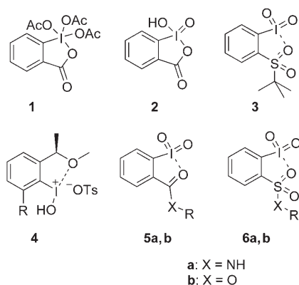
Scheme 1. Cyclic and pseudocyclic hypervalent iodine reagents.
